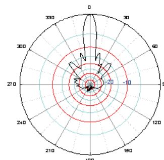
H-Plane Radiation Pattern
