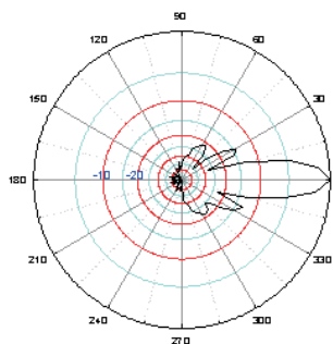
E-Plane Radiation Pattern
